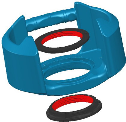
DOUBLE CLAMPING RINGS SYSTEM
